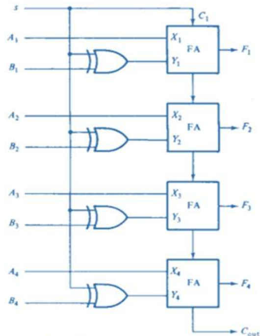
Figure 9-10 4-bit adder/subtractor circuit
